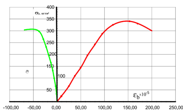
Figure. Stress-strain diagram of basalt fiber-reinforced concrete under compression.
